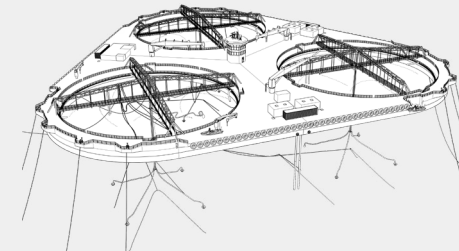
FARM-MAX
